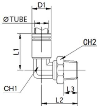
Dimensions of SPL 06-N01 Male Elbow Connector | Stainless Steel Push to Connect Fitting
